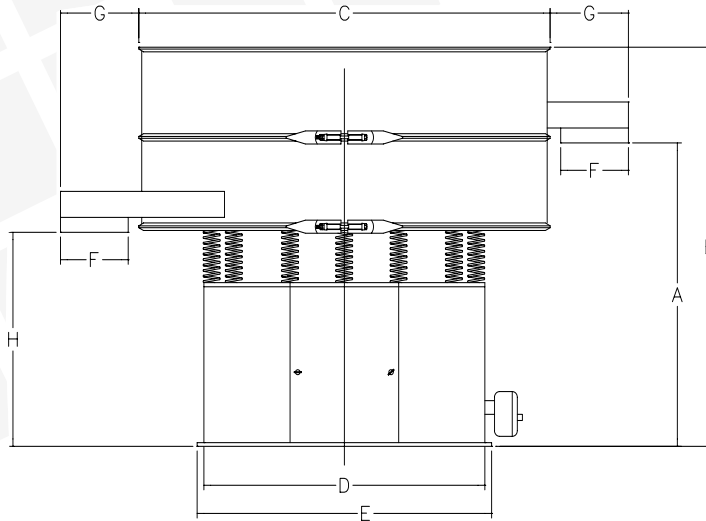
SHAKER SCREEN OUTLINE DIMENSIONS
